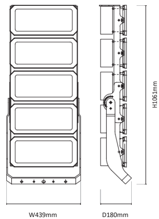
W439mm
