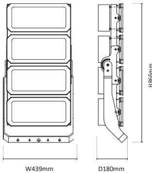
W439mm
