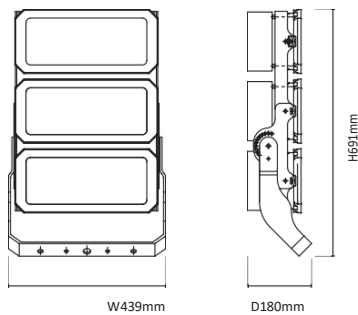
W439mm
